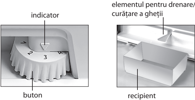
Figura 4 – Buton
